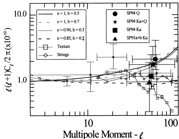
FIG. 2.—Band power estimates ( \pm 1 \sigma ) as given in Table 1 compared to a variety of theoretical power spectra and other recent low- \ell measurements. Reading from low \ell to high \ell , the other measurements include COBE, the Far-Infrared Survey, Tenerife, and SK93. The higher \ell measurements have not been included for clarity's sake but can be found in Bond (1994) along with complete citations. The horizontal error bars represent the FWHM of the given window function. The theoretical power spectra were provided by Steinhardt (1994).
