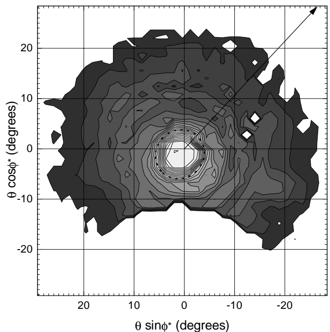
Fig. 17. Beam pattern mapping of the 1465 MHz backfire-fed GEM antenna, in twenty 1-dB steps and at a pixel resolution of at 1.6^\circ , using the passage of the Sun through the Z = 30^\circ scan circles of the antenna on the 29-th of September 1999 in Cachoeira Paulista, Brazil. The \phi^* angle of the pattern is measured counterclockwise from the ordinate axis and corresponds to \phi - 180^\circ in the coordinate system of Fig. 7b while the elevation of the Sun is given by 60^\circ - \theta \cos \phi^* . The arrow indicates the major axis alignment of the 10-dB elliptical contour toward the larger component of the double-lobed structure in Fig. 7b
