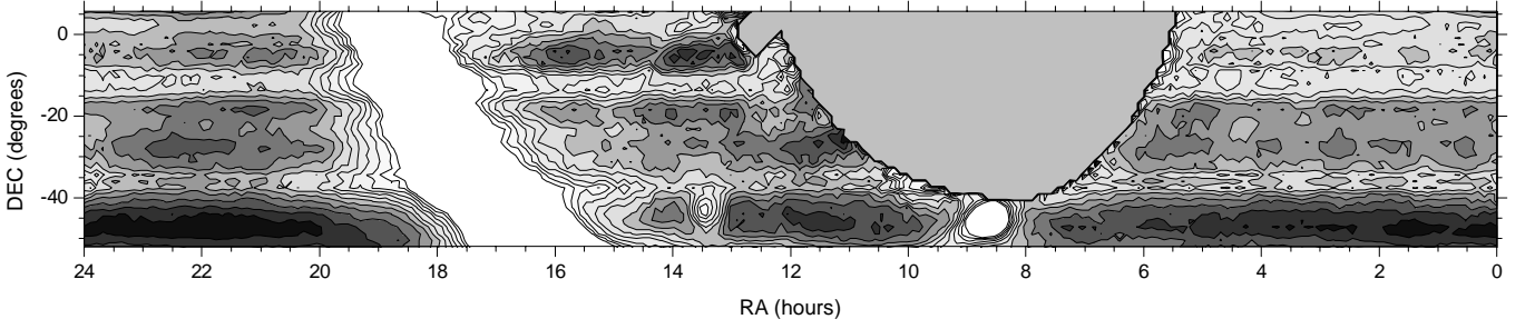
Fig. 2. A sky map at 1465 MHz of a 60^\circ declination band obtained with the GEM experiment in the Southern Hemisphere using only a rim-halo protection and assuming a uniform baseline level across the sky (Epoch 2000.0 coordinates). The pixelization is 1.6^\circ and the antenna temperature range extends 1.5 K above the lowest temperature in 12 equally-spaced contours in order to enhance the distribution of Galactic radiation away from the Galactic Plane
