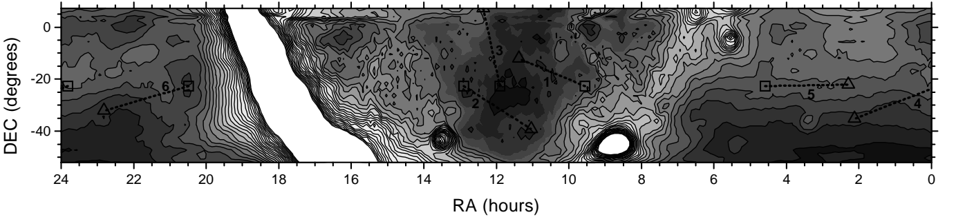
Fig. 3. A GEM map at 1465 MHz of the same sky region as that in Fig. 2 (same baseline assumption and pixel size), but using data obtained after the wire mesh screen had been added to the shielding configuration of the antenna. The antenna temperature ranges also over 1.5 K above the lowest temperature, but the contour levels are spaced more tightly (60 mK). Marked locations denote the sky directions of the 6 test measurements discussed in Sect. 5
