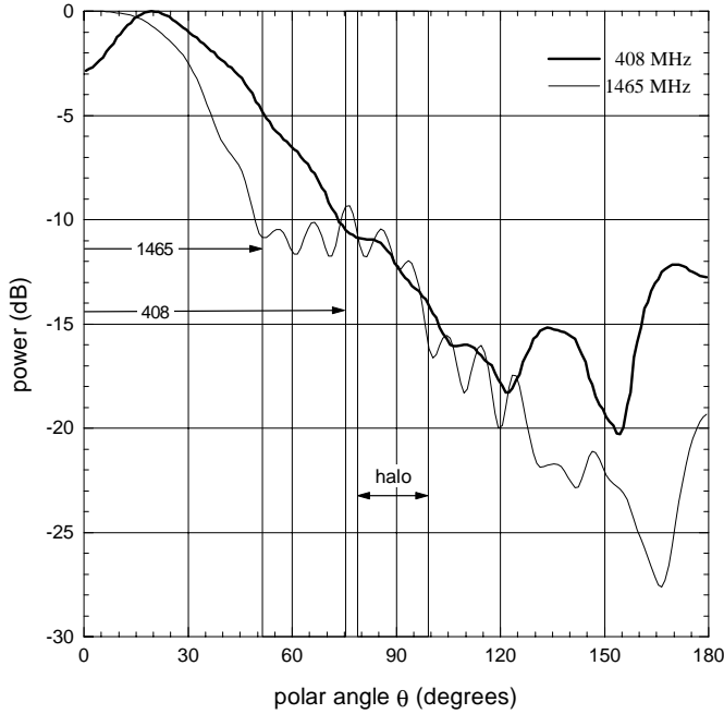
Fig. 8. Polar diagrams of the 408 MHz and 1465 MHz feed patterns using the mean backfire response in the \phi -plane. Vertical reference lines delimit the sidelobe structure within the field of view of the halo and the width of the assumed main beams
