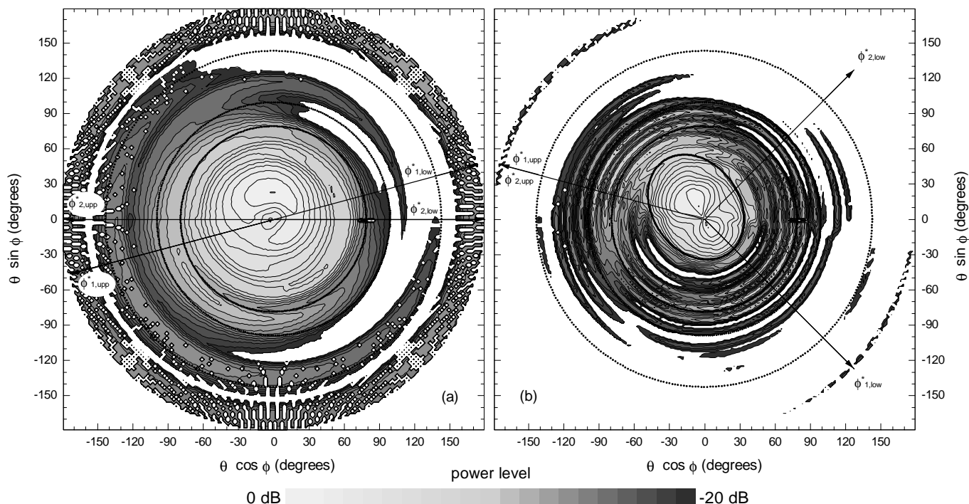
Fig. 7. Diagram representations of the backfire power patterns at a) 408 MHz and b) 1465 MHz in a coordinate reference frame centered on the transmitter. Three concentric circles have been superimposed on the diagrams to illustrate the opening angles of the ground shields: the boundary of the dish itself at \theta = 78.9^\circ , the rim-halo at \theta = 99.2^\circ and the farthest lying location on the upper edge of the fence at \theta = 142.9^\circ when Z = 45^\circ . The 10-dB level at 1465 MHz is mostly contained inside the elliptical contour. Arrows indicate the \phi^* ( \equiv 180^\circ - \phi ) orientations of the feed for generating the upper (upp) and lower (low) envelopes in Figs. 10-13. The subindex number denotes the number of shields accounted for (1: only the rim-halo, 2: both halo and fence)
