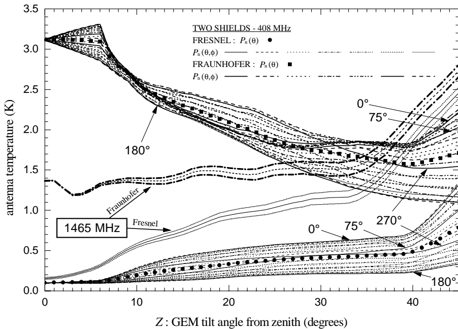
Fig. 11. Predicted antenna noise temperature due to transmitted and diffracted ground radiation in the double-shielded GEM experiment at 408 MHz. Two additional triple-sets of profiles have been included to show the Fresnel and Fraunhofer estimates at 1465 MHz for \phi = 12^\circ using a 7.91^{(+0.35}_{-0.32)} -dB attenuating fence and raised 80 cm above the ground as discussed in Sect. 5.2. Legend and label explanations are as in Fig. 10
