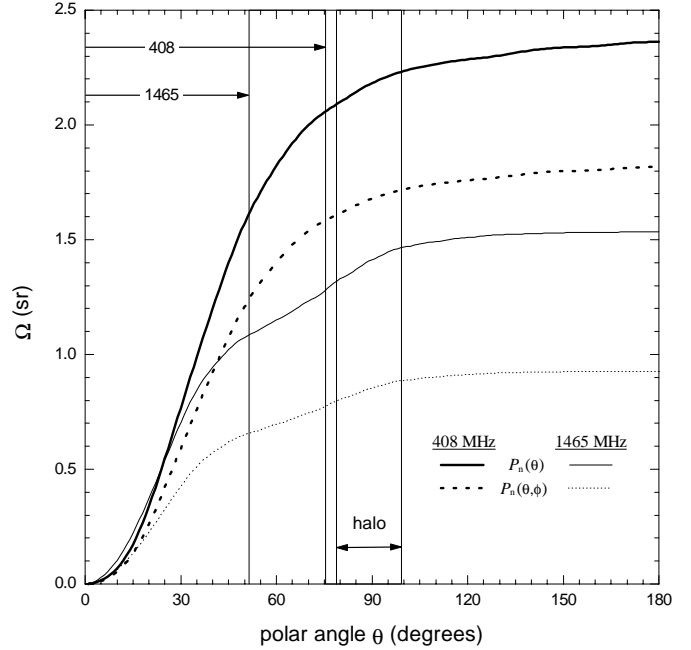
Fig. 9. Antenna solid angle growth with polar angle for the beam patterns in Fig. 8 and for the full 3-d measured response of the backfire feeds. The vertical lines are as in Fig. 8
