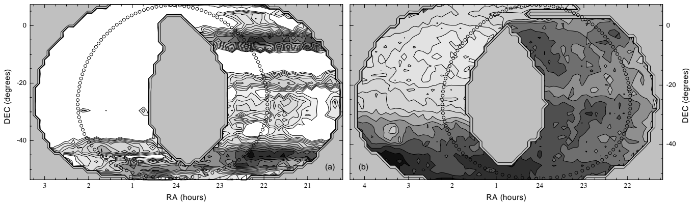
Fig. 5. Maps of the sky regions revealed by the circularly scanning technique of the GEM experiment at 1465 MHz, a) before and b) after the construction of the fence, and the distribution of the alt-azimuth sky bins used in the sampling of the signal displayed in the antenna temperature profiles of Figs. 4a,b. Map a) consumed 2.29 hours of observational time and Map b) 2.18 hours. Both maps are given at a 1.6^\circ pixel-resolution and their antenna temperatures range in 12 contour steps of 60 mK above their respective minimum values
