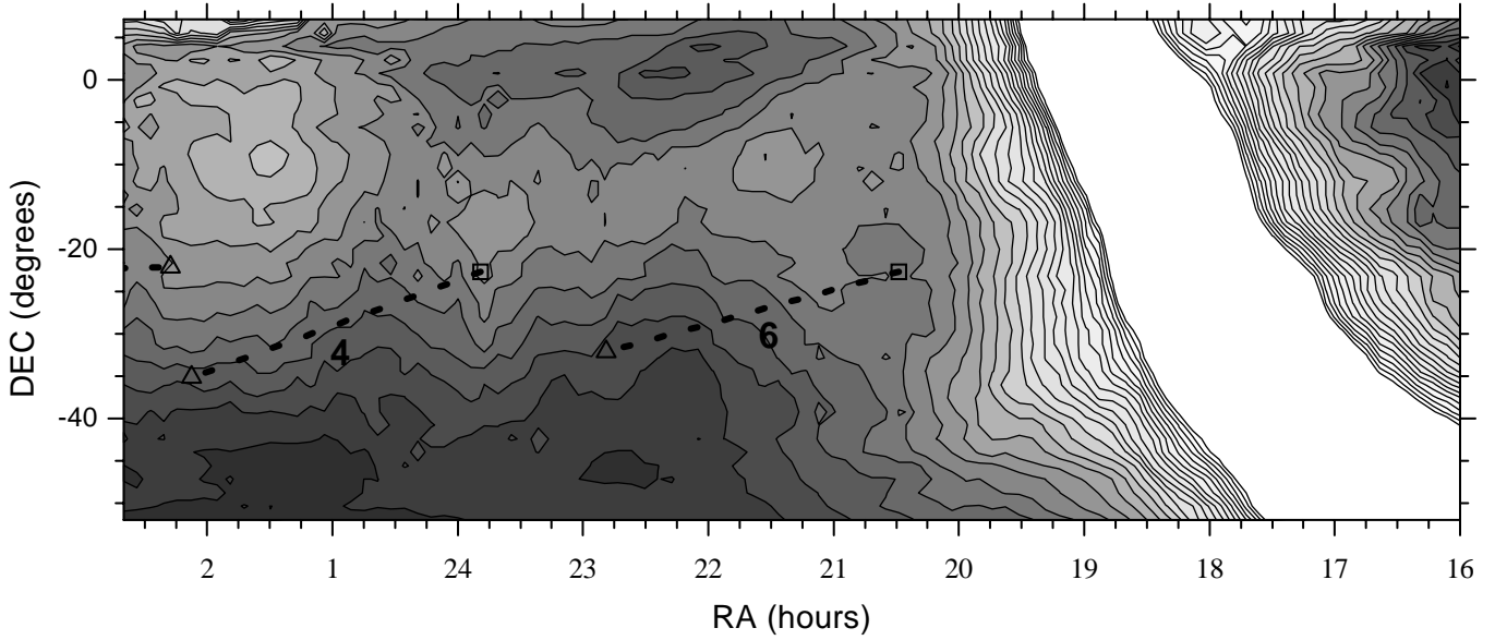
Fig. 15. Destriped partial map at 1.6^\circ -pixel resolution of the high-sampled sky regions displayed in the declination band of Fig. 3. The antenna temperature range is 1.5 K in 60 mK contour steps. Squared and triangular symbols denote, respectively, the sky directions of the paired Z = 90^\circ and Z = 60^\circ observations for the test measurements
